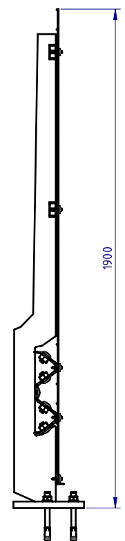
RhinoStop® Screen Type 3, 1900mm High
